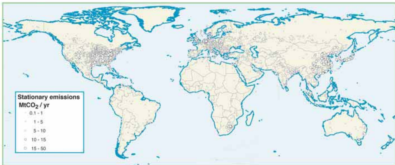
Figure SPM.6a. Global distribution of large stationary sources of CO 2 (Figure 2.3) (based on a compilation of publicly available information on global emission sources; IEA GHG 2002)
